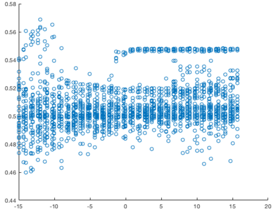
ROC AUC score vs log10(C)
